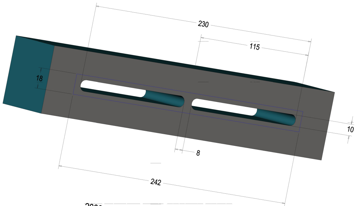
2000 SLIMLINE VENT ROUTING DETAIL
